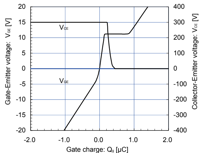
Dynamic Gate Charge (typ.) V_{CC} = 300\text{V} , I_C = 200\text{A} , T_J = 25^\circ\text{C}
