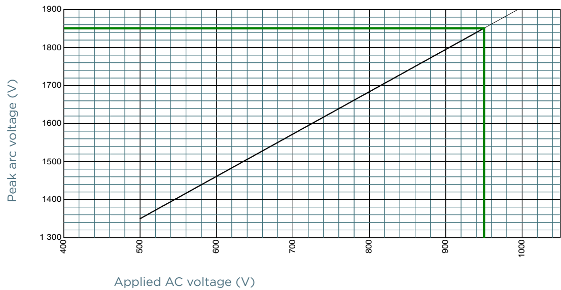
Size 73 aR 950V
