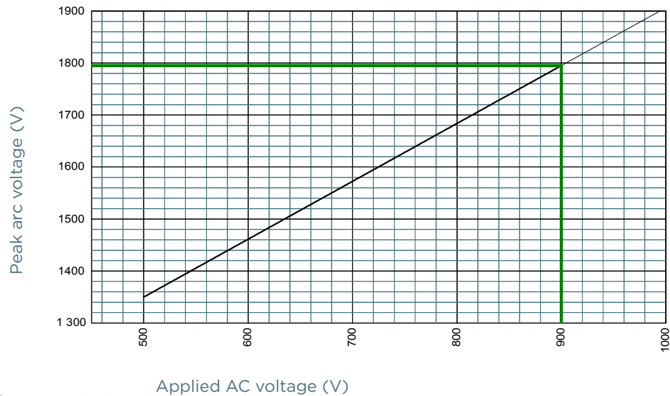
Size 73 aR 950V
