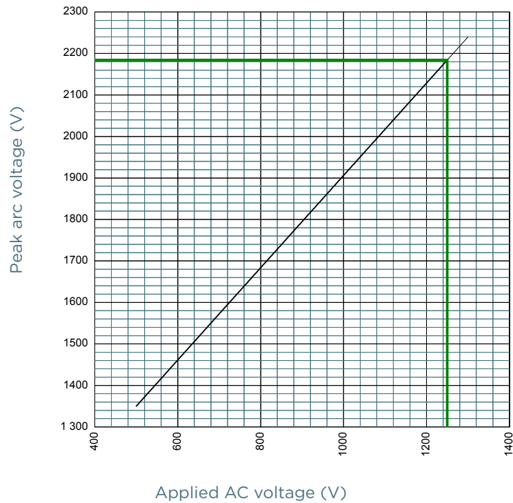
Size 73 aR 1250V
